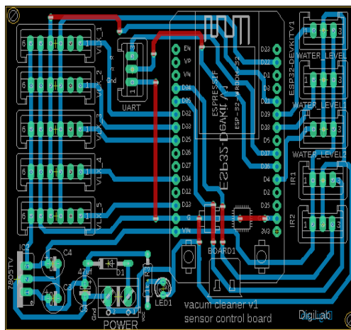
Figure 15. ESP32_vacuum_board
